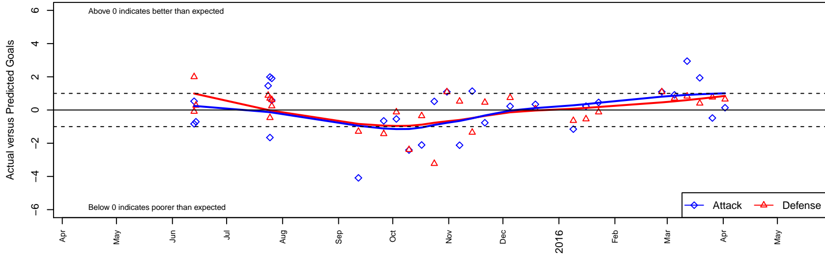
MIFC Thunder G01 Dots are actual minus expected GF (blue circles) and GA (red triangles). Blue line is smoothed change in attack strength. Red is smoothed change in defense strength.
